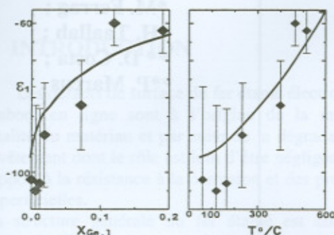
Fig.5 real part of \epsilon \text{Ga}_{77}\text{Ga}_{23} plotted versus x_{\text{Ge},1} in the left part and versus T according to the diagram in the right part. Full symbols: ellipsometric measurement at 1107nm.
