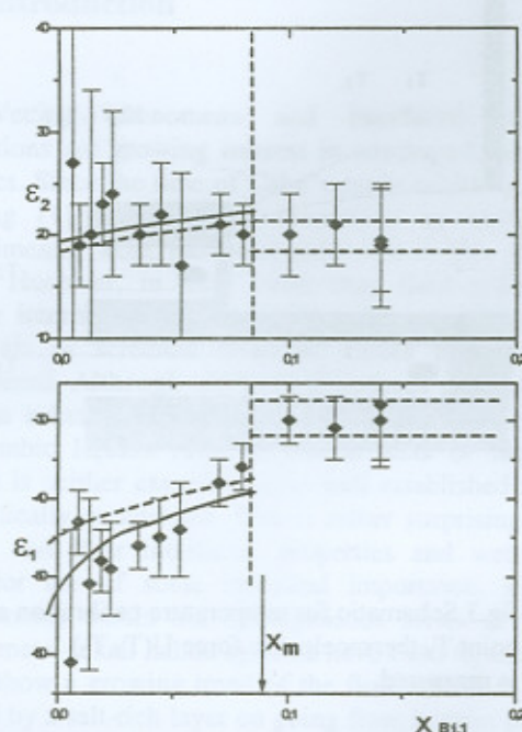
fig.4 full symbols: ellipsometric results of \epsilon_1 and \epsilon_2 at 600nm of \text{Ga}_{85}\text{-Bi}_{15} for details see text.
