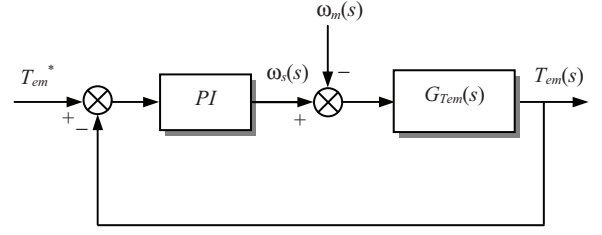
Fig. 2. Closed-loop control of electromagnetic torque.
