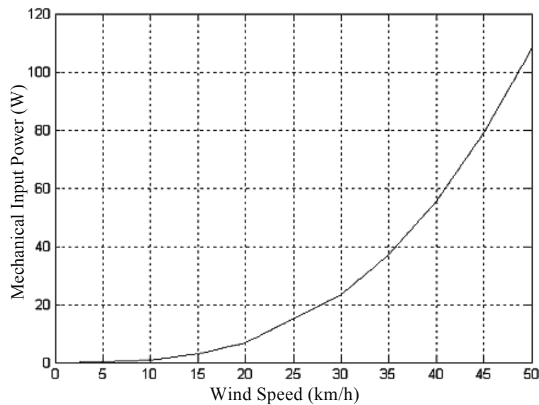
(b) Available input power (blades rotation) versus wind speed.
