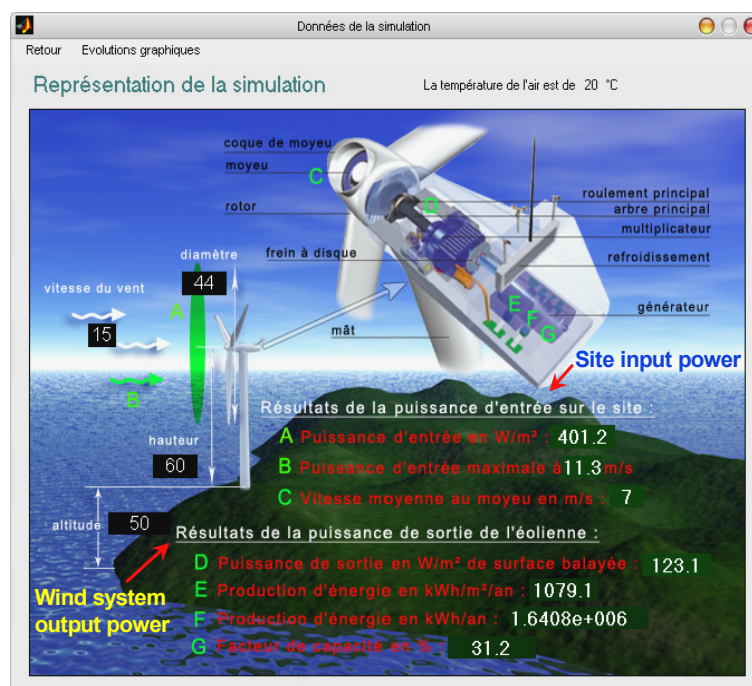
Fig. 12: Simulation window
