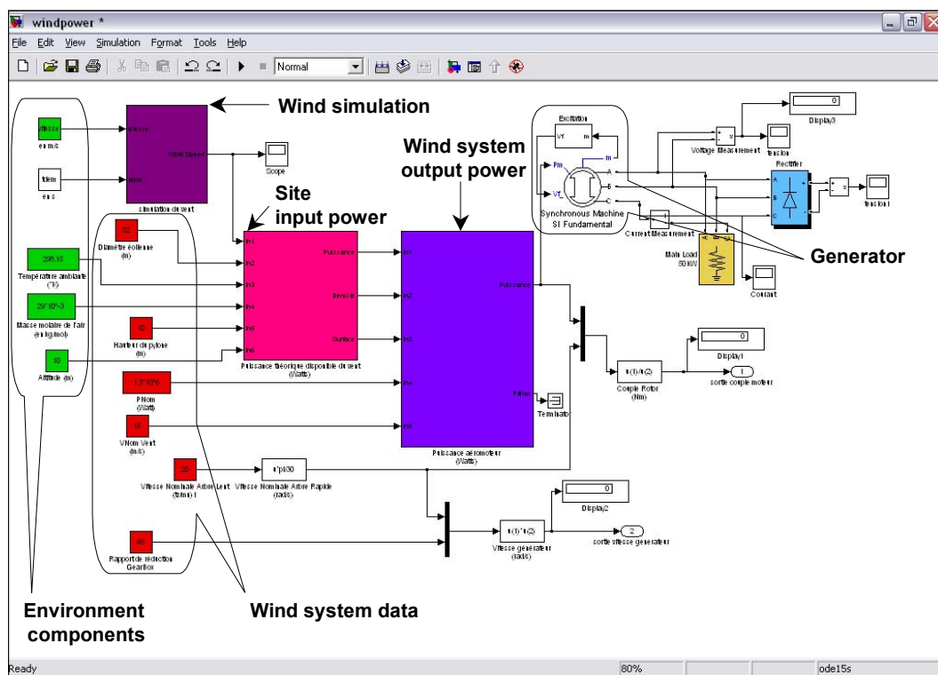
Fig. 6: Wind turbine simulation
