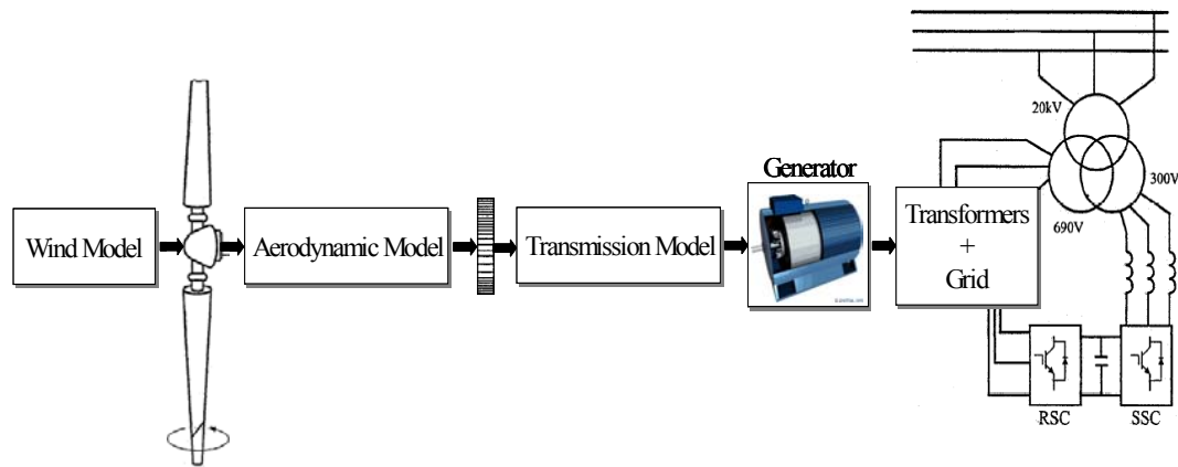
Fig. 5: Simplified scheme of wind turbine model
