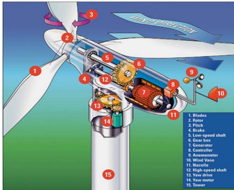
Fig. 3: Cutaway of a wind turbine nacelle
