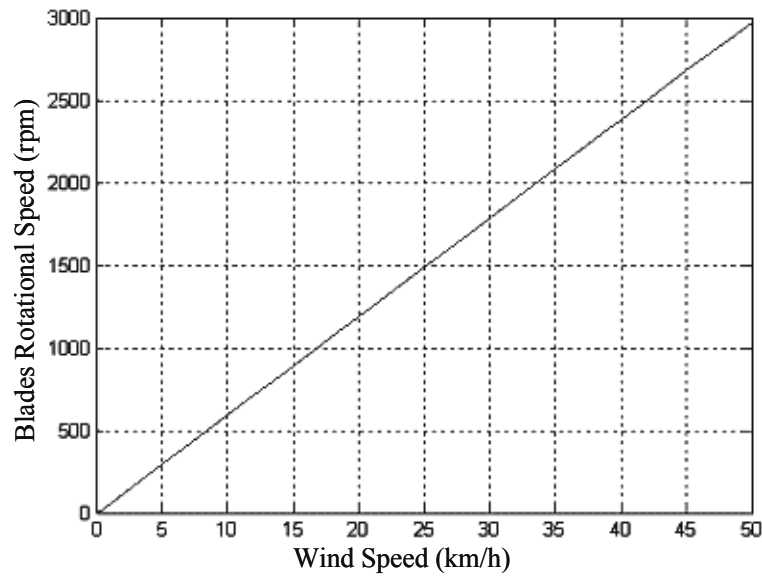
(a) Blade rotational speed versus wind speed.
