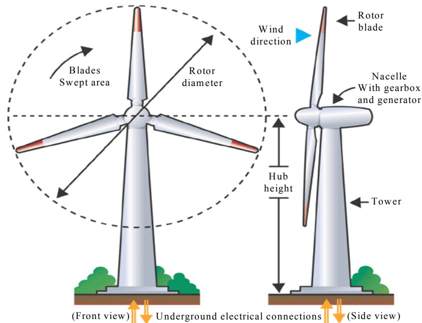
Fig. 7: Wind energy system schematic
