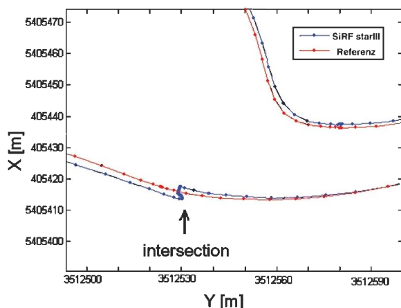
Fig. 9 Error at intersection for SiRF receiver.
